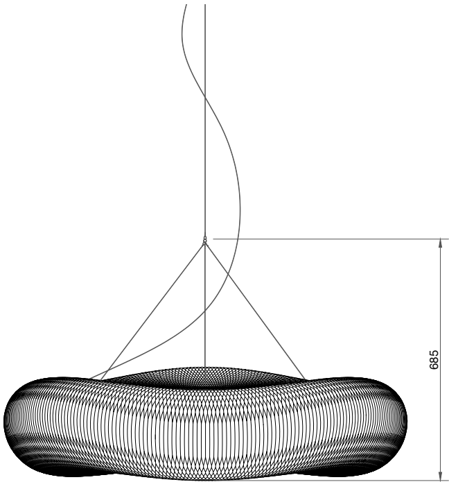
ELEVATIONS *
