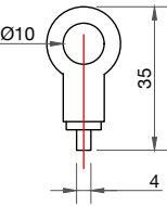
ELEVATION OPTION C · GRIPPER RING
