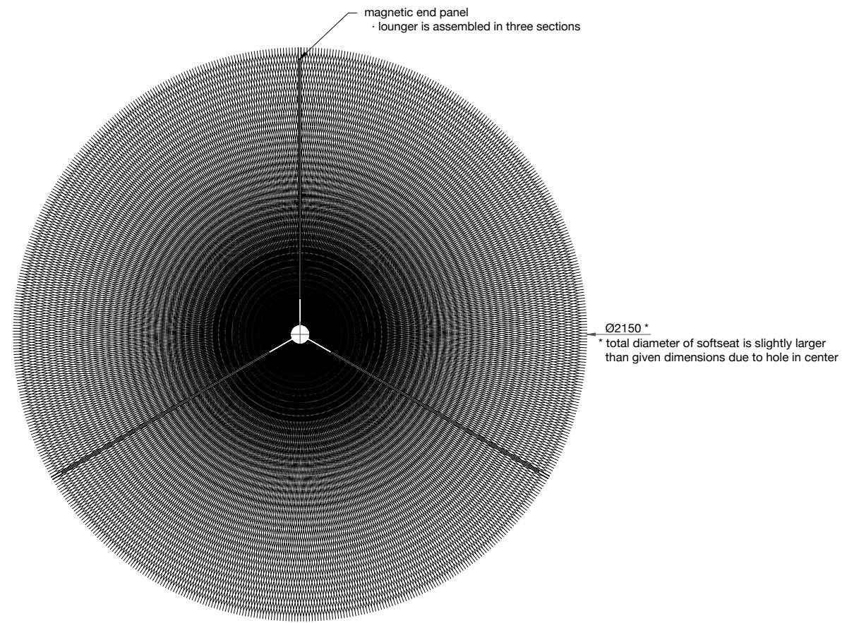
PLAN · softseating - lounger
