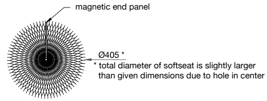
PLAN · softseating - fanning stool + table
