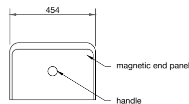
ELEVATION · COMPRESSED
