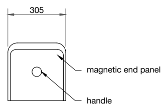
ELEVATION · COMPRESSED
