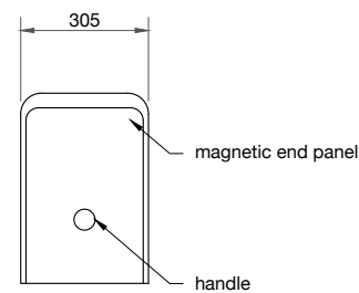
ELEVATION · COMPRESSED
