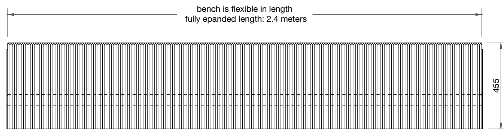
ELEVATION · softseating - bench
