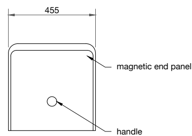
ELEVATION · COMPRESSED
