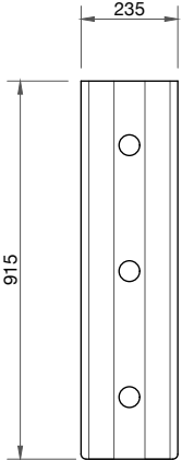
ELEVATION · OPEN END PANEL
