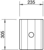
ELEVATION · OPEN END PANEL
