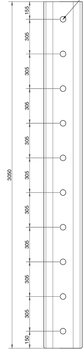
ELEVATION · UNFOLDED END PANEL (RADIUS-CUT CORNERS)
