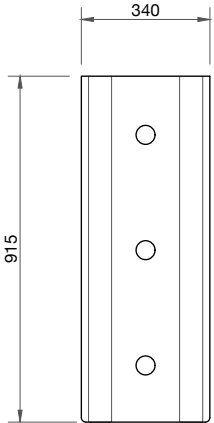
ELEVATION · OPEN END PANEL
