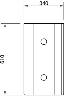
ELEVATION · OPEN END PANEL
