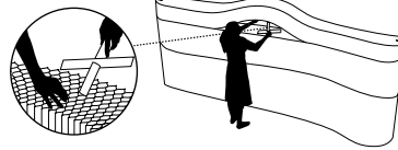
peg + strip reinforce the connection between horizontal layers of softblock
