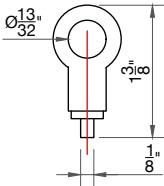
ELEVATION OPTION C · GRIPPER RING
