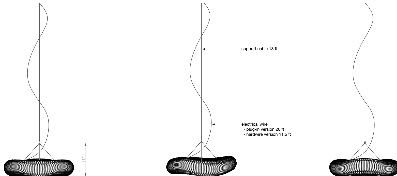
ELEVATIONS *
