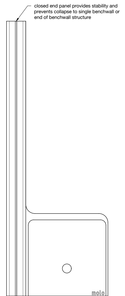
ELEVATION · CLOSED END PANEL
