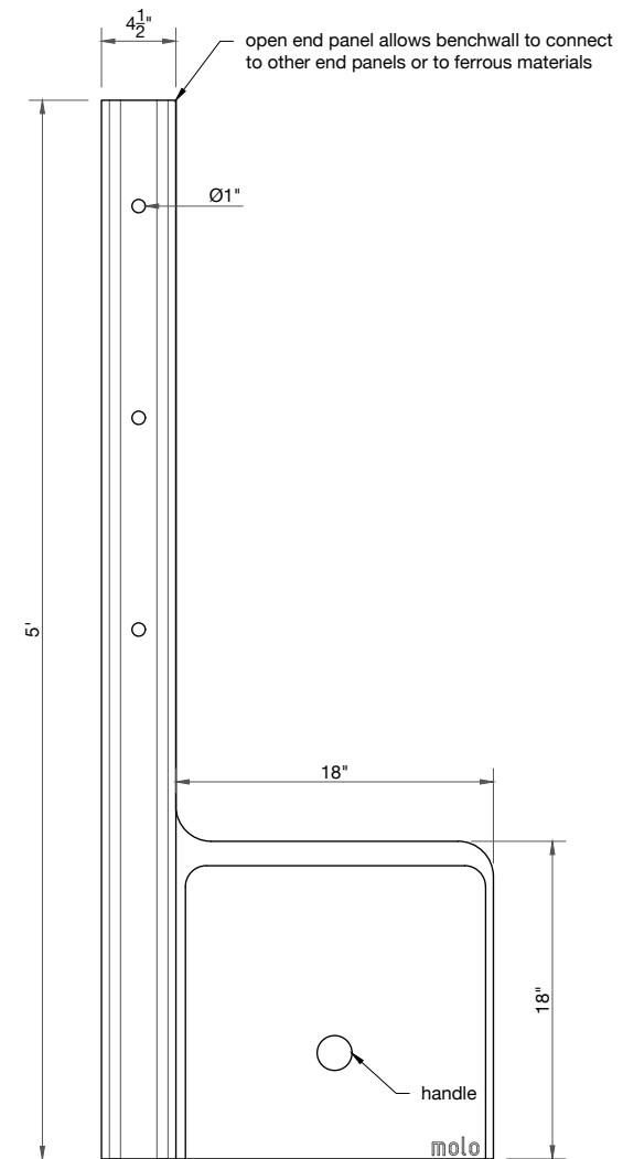
ELEVATION · OPEN END PANEL
