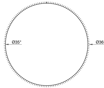
PLAN · WOOL FELT PAD
