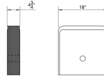
ELEVATION · COMPRESSED VIEWS
