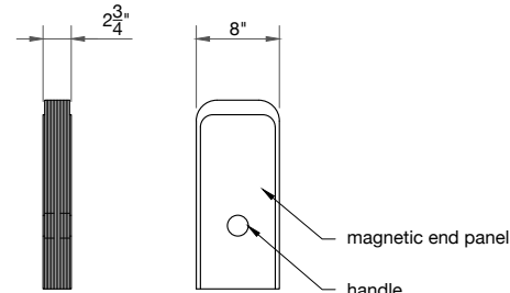
ELEVATION · COMPRESSED VIEWS
