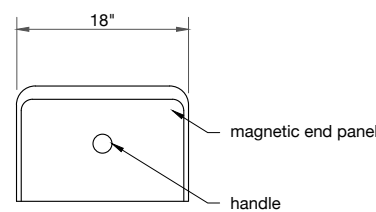
ELEVATION · COMPRESSED
