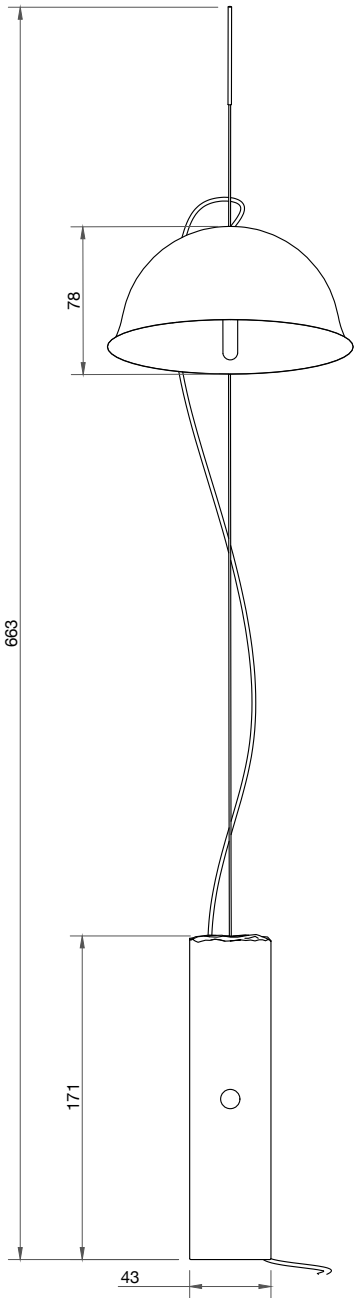
ELEVATION · FRONT
